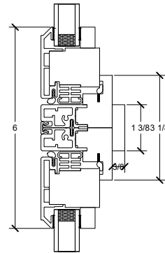
Horizontal Mull
