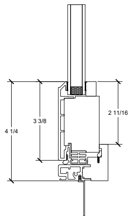
Big Bottom Rail
