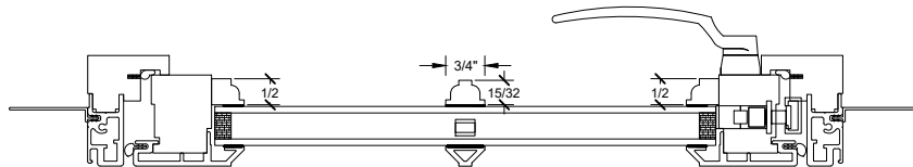
Long Bead Interior SDL—Long Bead Interior Glaze Bead/Bevel Bead Exterior
