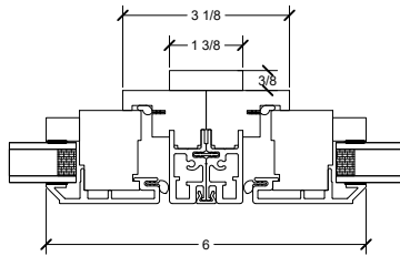
Vertical Mull
