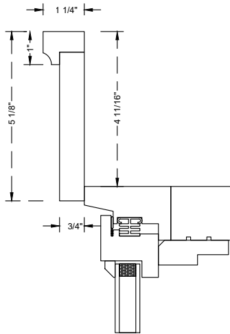
1 x 5 Casing w/ Backband
