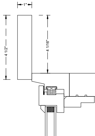
5/4 x 5 Casing
