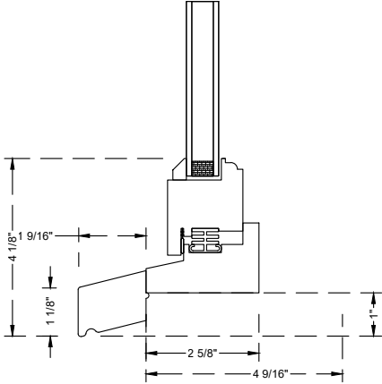
Subsill (2814)
