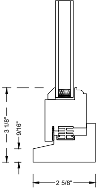
Standard (No Sub Sill)
