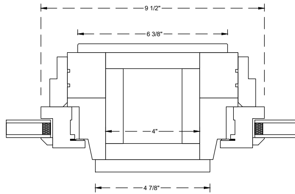
4" Spread Mull
