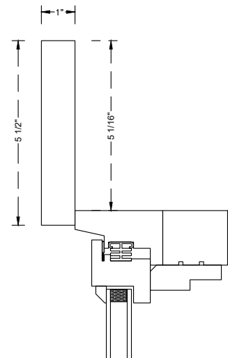
5/4 x 6 Casing
