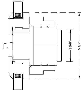
Standard Horizontal T-Mull
