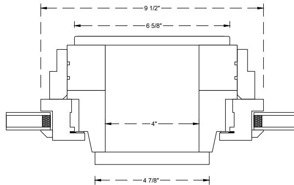
4" Space Mull
