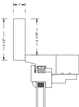
5/4 x 4 Casing
