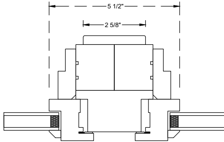
Standard Vertical T-Mull
