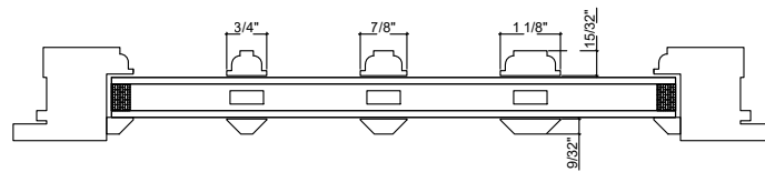
1/2" Long Bead Interior/Bevel Bead Exterior
