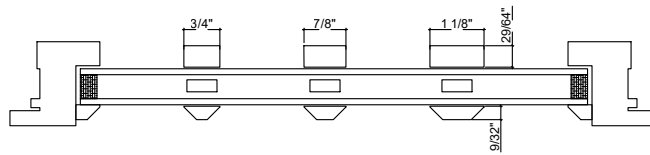
Square Detail Interior/Bevel Bead Exterior
