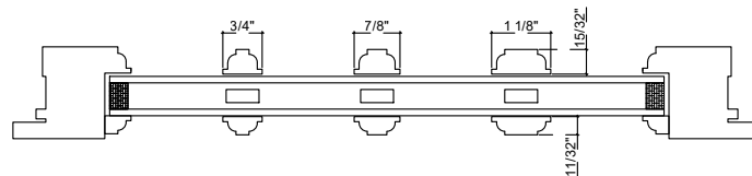
1/2" Long Bead Interior/Long Bead Exterior
