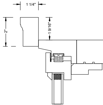
Brickmold Casing
