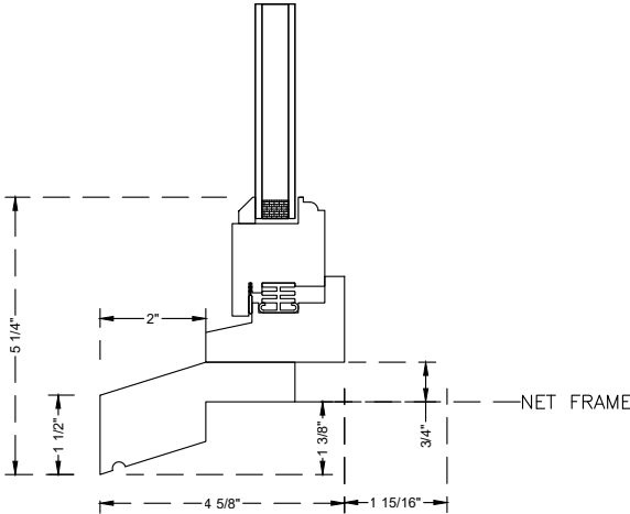
True Subsill (2816)
